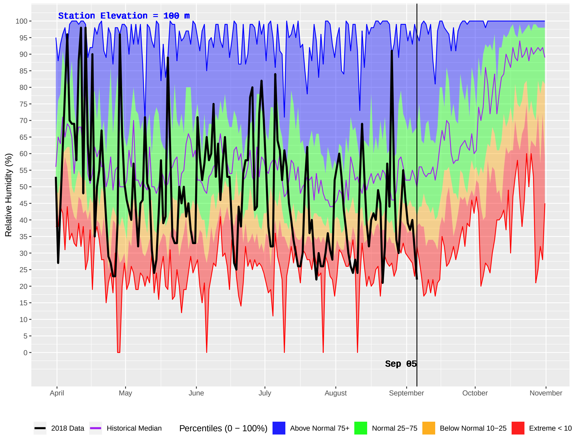
BEAVER CREEK (37) : Historical (1987–2016) and Current (2018) Daily Relative Humidity
